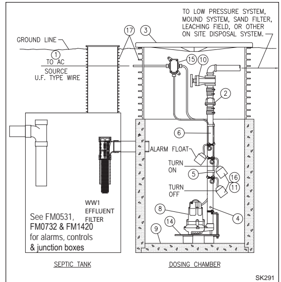
TYPICAL EFFLUENT INSTALLATION
