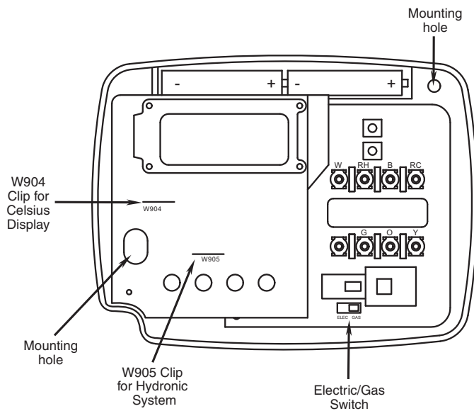
Figure 1. Thermostat
