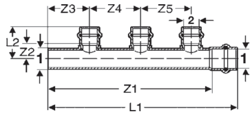
Copper ProPress Manifold 3-Outlet (open) P x FTG x P - Model 2945
