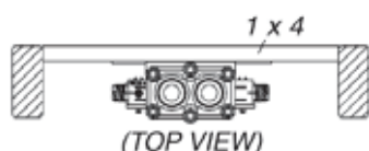
1 x 4s attach at the back, inside the studs, and the MANABLOC is centered between the studs.
