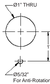
EC-3100 & EC-3102 MOUNTING HOLE DIAGRAM
