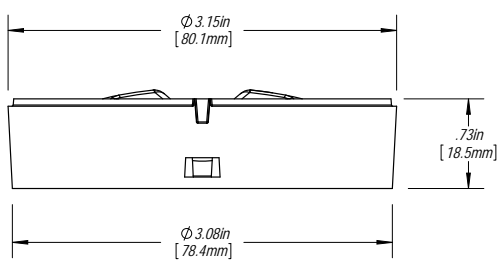
Housing (No Gasket)
