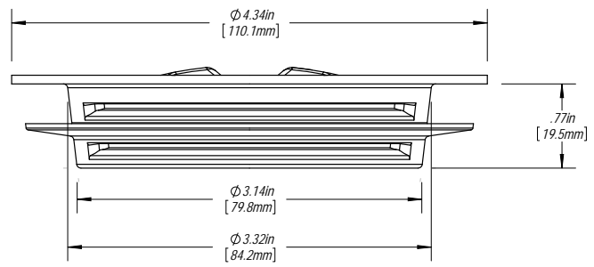
Housing & Gasket
