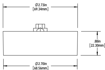
Housing (No Gasket)
