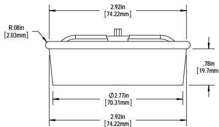
Housing & Gasket A
