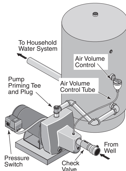
Figure 5: Standard Tank Connections
