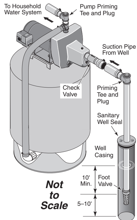
Figure 2: Cased Well Installation
