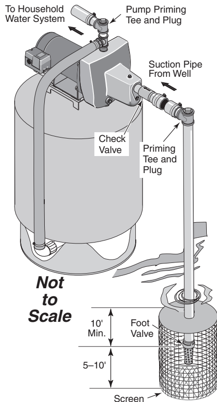
Figure 3: Surface Water Installation
