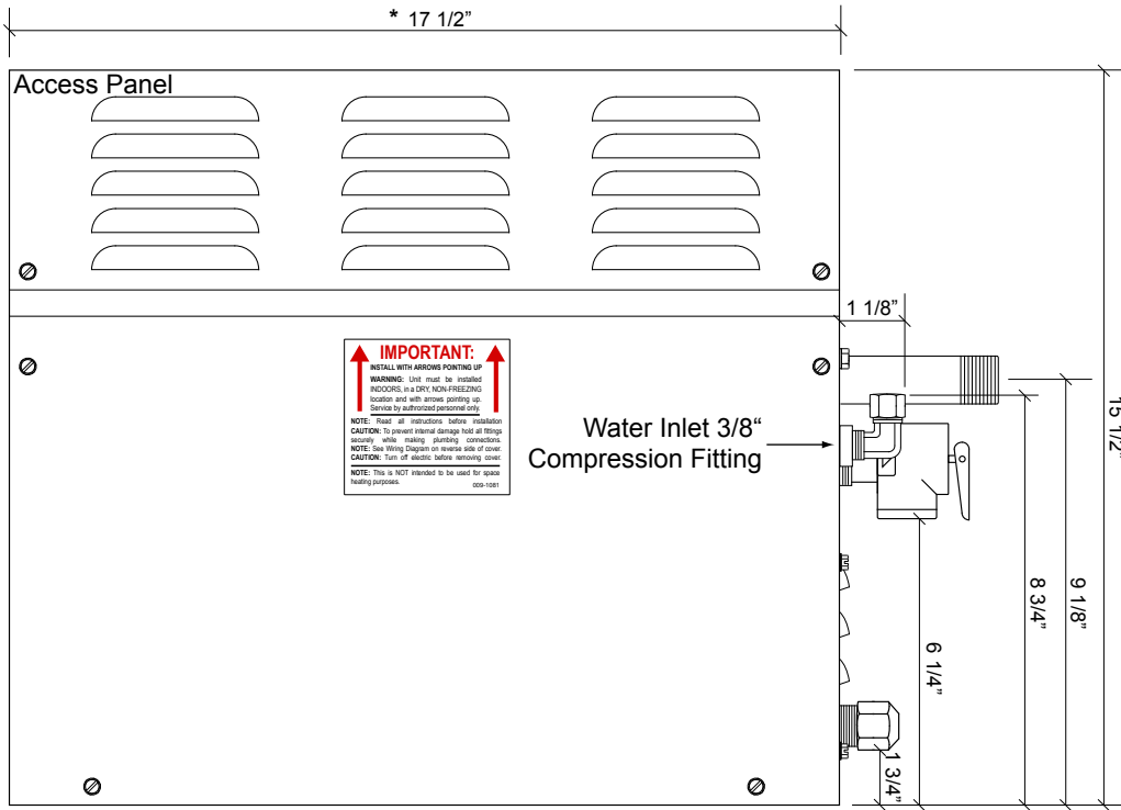
Front Access
