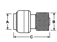
Stop Connector Dimensions (Chrome Plated)
