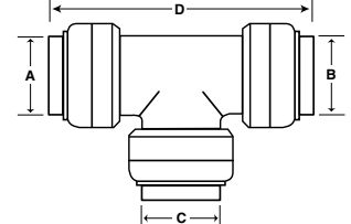
Tee Dimensions
