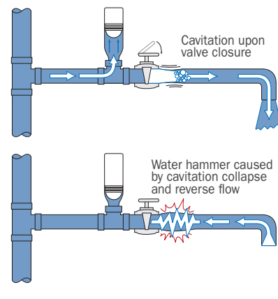
Fig 3: Shut-off valve in MIDDLE of long pipe run
