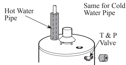
Typical vertical piping arrangement
