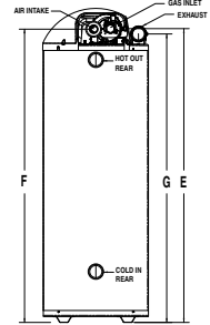
REAR
