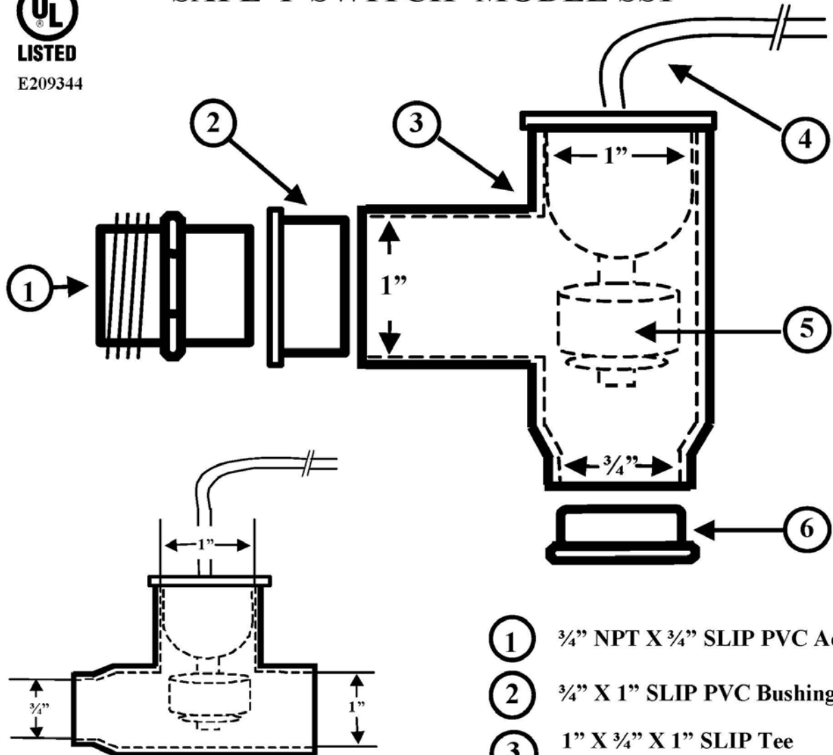
HORIZONTAL APPLICATION
