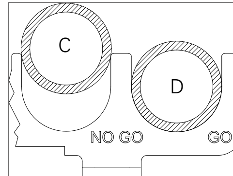
Figure 4 – Good Connections; crimped ring fits in "GO" slot C) Crimped ring does not fit in "NO GO" slot – ring is oversized; D) Crimped ring does fit in "GO" slot – ring is oversized.
