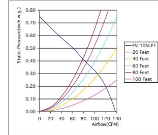
FV-10NLF1 120 CFM 4" Duct
