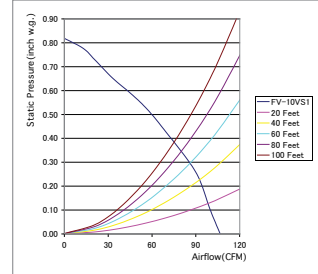
FV-10VS1 100 CFM 4" Oval Duct
