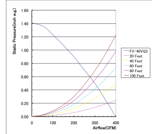
FV-40VQ3 380 CFM 6" Duct
