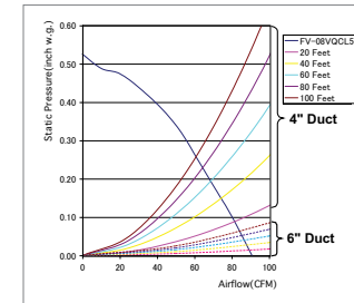
FV-08VQL5 80 CFM 4" or 6" Duct
