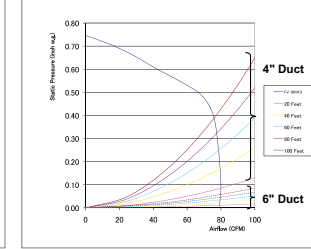
FV-08VK3 80 CFM 4" or 6" Duct
