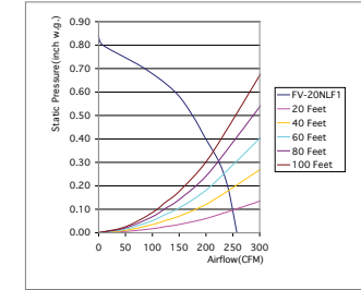
FV-20NLF1 240 CFM 6" Duct
