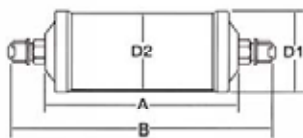
Flare Connection
