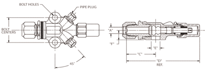
4-BOLT MOUNTING STYLE-SOLDER TYPE-FLAT GASKET SURFACE-PLASTIC CAP
