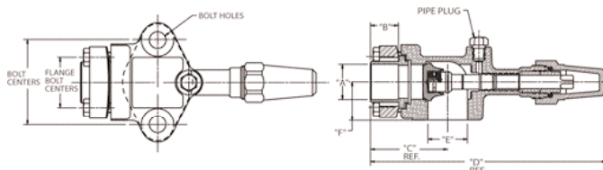
FLANGE UNION-SOLDER TYPE-PLASTIC CAP
