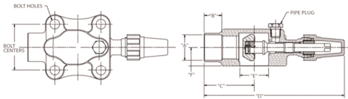
DOUBLE PORT-SOLDER TYPE-STEEL CAP
