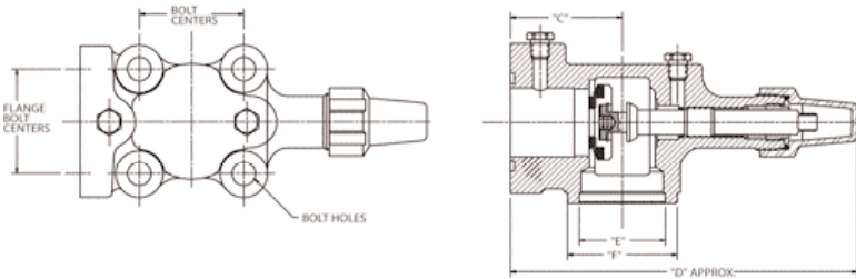
4-BOLT-CAST IRON COMPRESSOR VALVES WITHOUT FLANGES
