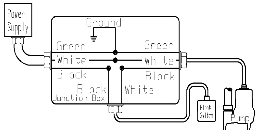
Fig. B – Direct Wiring of 120V or 208-230V Single Phase, Automatic Pumps
