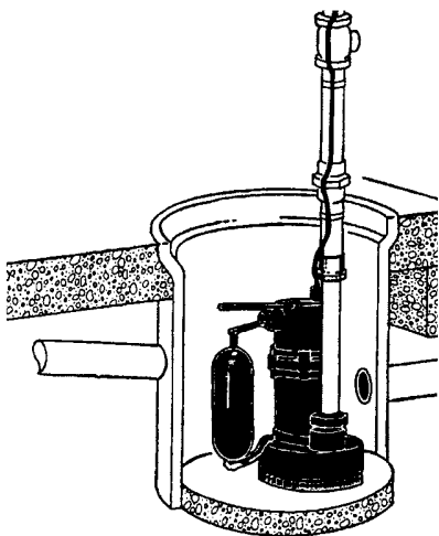
Typical Installation
