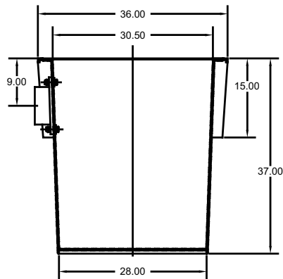
30" x 36" Basin
