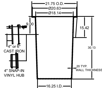
18" x 30" Basin
