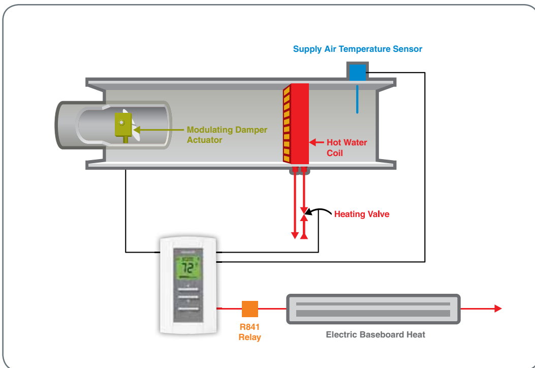
TB980B1005: Cooling Only Pressure Dependent VAV Zone Reheat and Electric Baseboard Heat
