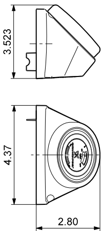
Fig. 12 Timer dimensions, current version
