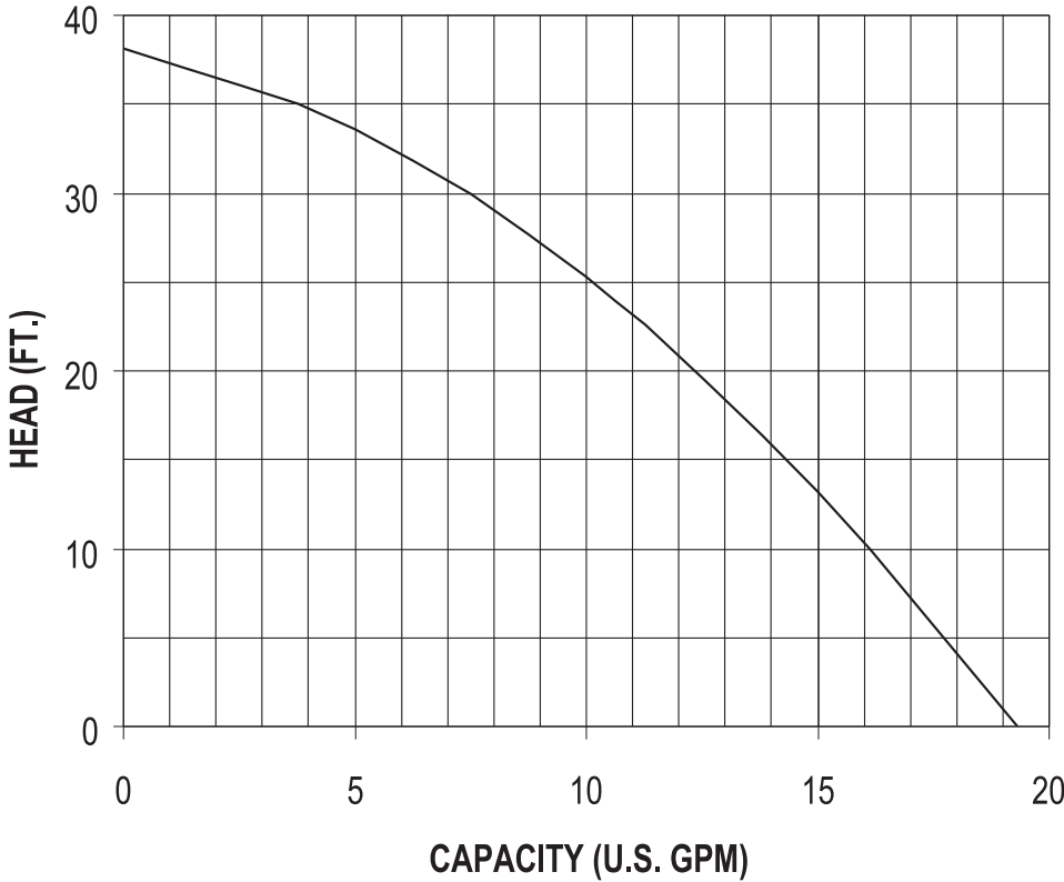
UP 26-120U Closed Systems, 60 Hz
