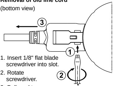
Fig. 1 Removal of old line cord
