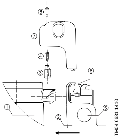
Fig. 3 Terminal box installation
