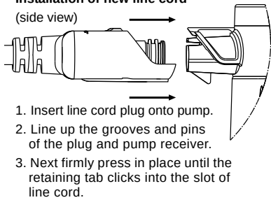
Fig. 2 Installation of new line cord
