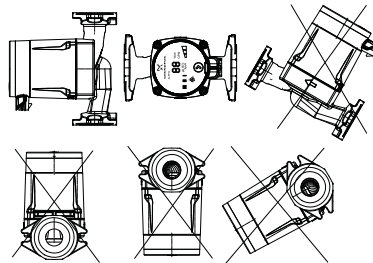
Fig. 2 Installation positions
