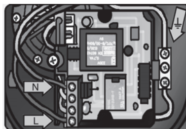
Fig. 10 Electrical connection
