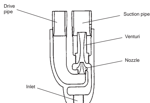
Fig. 3 Suction lift pressure boosting
