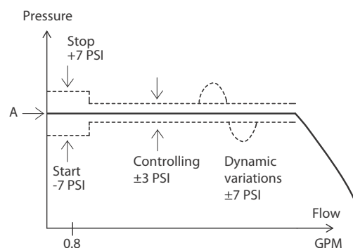
Fig. 5 System function
