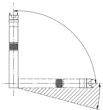
Fig. 8 Installation positions
