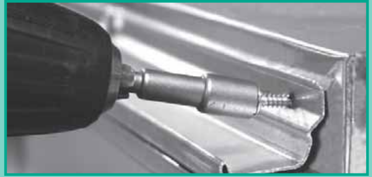
Drill Point Length Must Exceed Total Thickness
