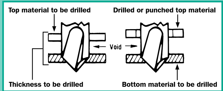
Drill Point Length Must Exceed Total Thickness
