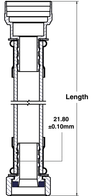
SharkBite® Water Heater Kit Dimensions
