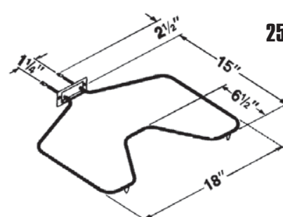
00701 2600w 240v Bake Element
