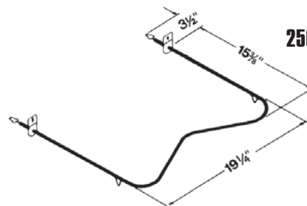
00631 2700w 240v Bake Element
