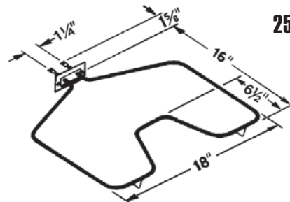
00651 3000w 250v Bake Element
