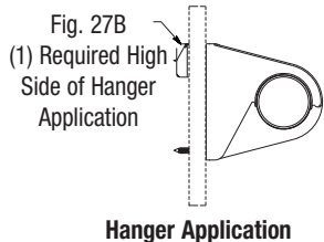
Hanger Application
