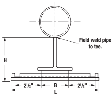
B3897 Front View
