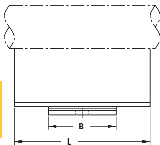
B3991-5 (shown) & B3991-10 Side View
