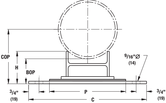
B3991-10 Front View
