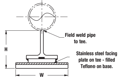
B3894 Front View
