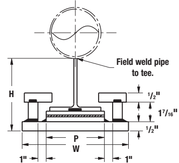
B3896 Front View
