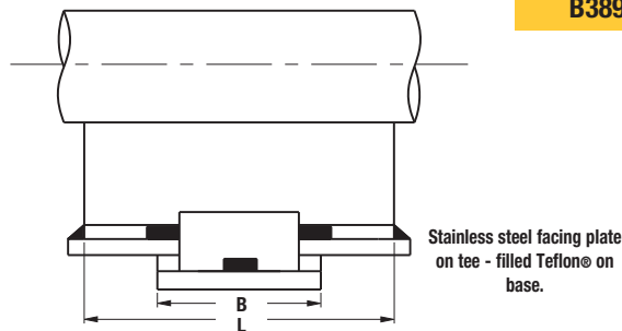
B3892 & B3895 Side View
