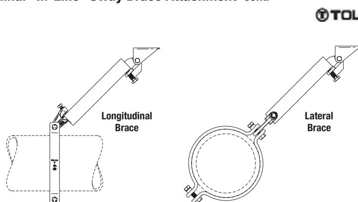
Fig. 4LA - Longitudinal “In-Line” Sway Brace Attachment cont.
