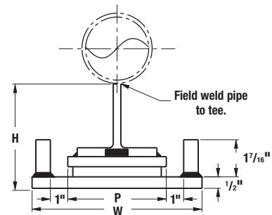
B3895 Front View
