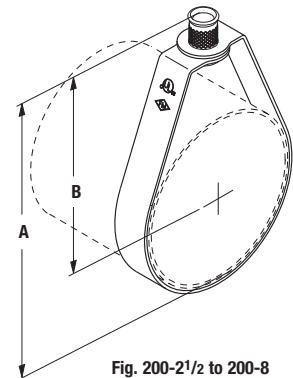
Fig. 200-2 1/2 to 200-8
