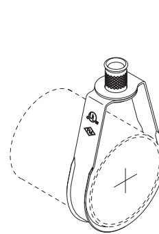
Fig. 200-1/2 to 200-2
