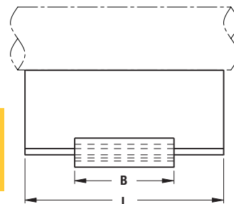
B3993-5 (shown) & B3993-10 Side View
