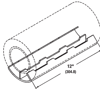
Sizes 12" (300mm) and larger
