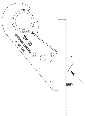
Hanger Application
