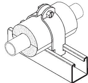
Strut Mounted
