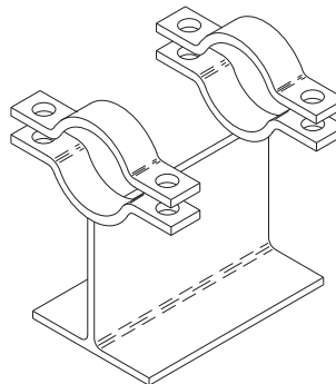
CL (standard slide with B3140 clamps)
