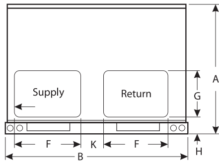
REAR
