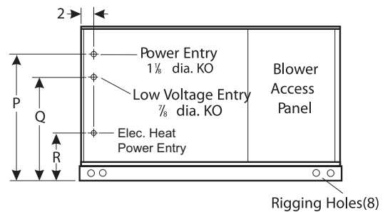
RIGHT SIDE
