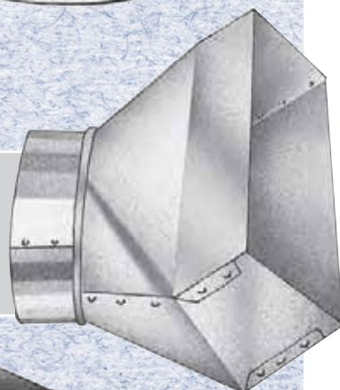
#243S 45° Register Boot
